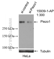
WB result of Piezo1 antibody (15939-1-AP; 1:300; incubated at room temperature for 1.5 hours) with sh-Control and sh-Piezo1 transfected HeLa cells.
