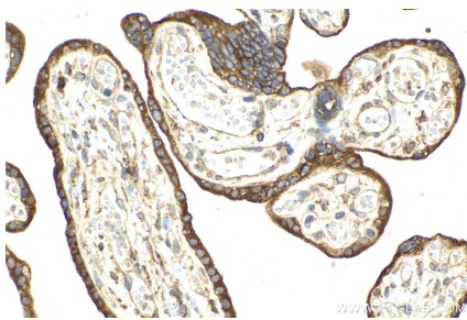
Immunohistochemical analysis of paraffin-embedded human placenta tissue slide using KHC2136 (STBD1 IHC Kit).
